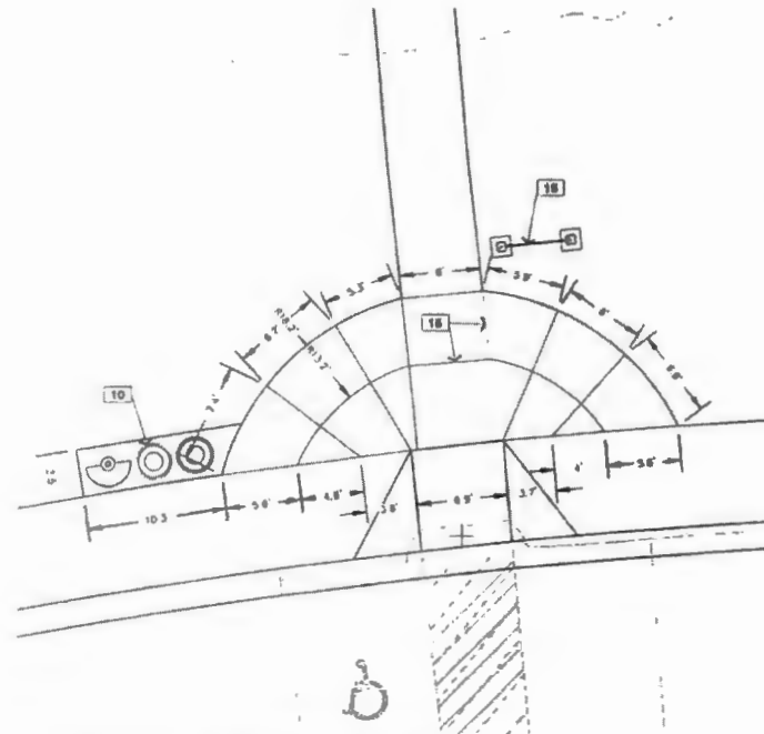
ADMINISTRATION BUILDING SIDEWALK PAVEMENT DETAIL SCALE 1/8" = 1'-0"
