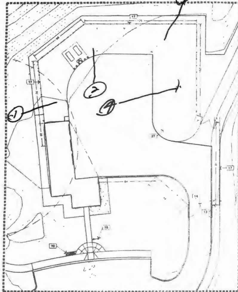
ADMINISTRATION BUILDING ENLARGEMENT SCALE 1/8" = 1'-0"
